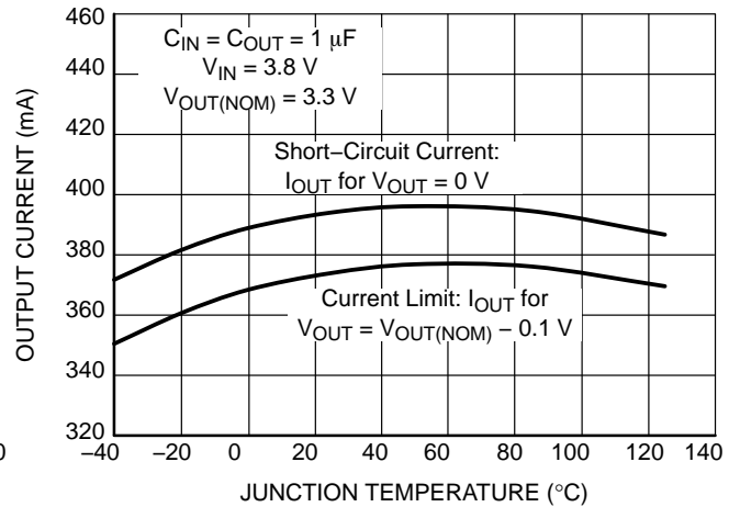
Figure 32. Short-Circuit Limit vs. Temperature V_{OUT} = 3.3\text{ V}
